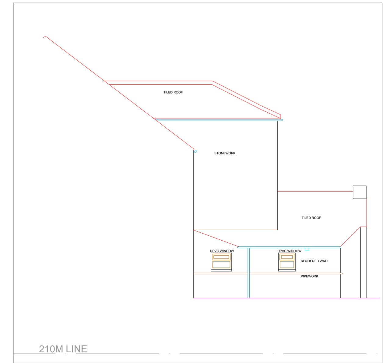
EAST ELEVATION 02 1:100 Scale
